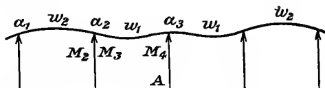
FIG. 149.—Continuous beam loaded to give maximum moment at a beam support.
