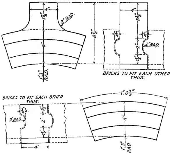
FIG. 134.—Plan and sections of fire-bricks.
