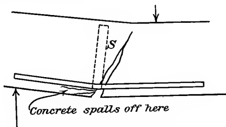
FIG. 47.—Spalling of concrete at under side of beam.
