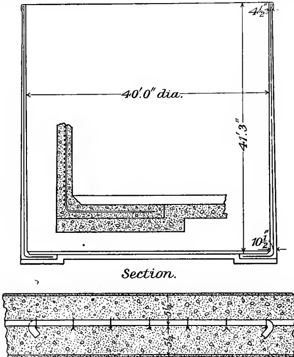
FIG. 119.—Detail of reservoir at Mittagong, N.S.W.
