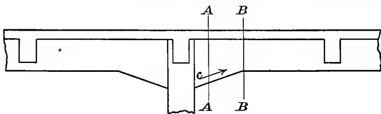
FIG. 54.—Haunches as reducing shearing forces.
