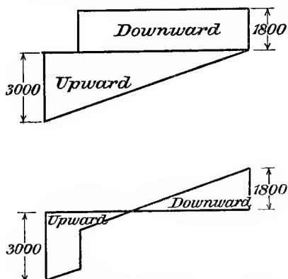
FIG. 131.—Unbalanced pressure on footing.
