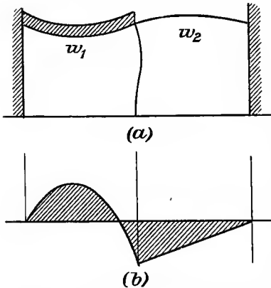
FIG. 69 (a) and (b).—Two spans, one loaded.
