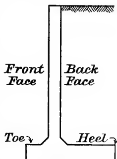
FIG. 125.—Terms used for retaining wall.
