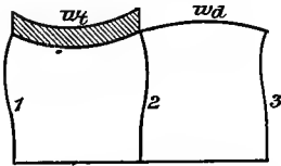
FIG. 80.—Two spans, one fully loaded.
