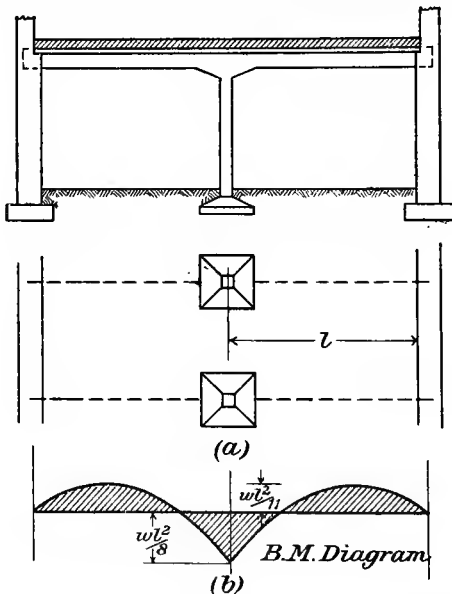
FIG. 64.—Continuous beams, freely supported at ends.
