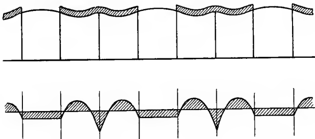
FIG. 67.—Two loaded spans alternating with one unloaded.
