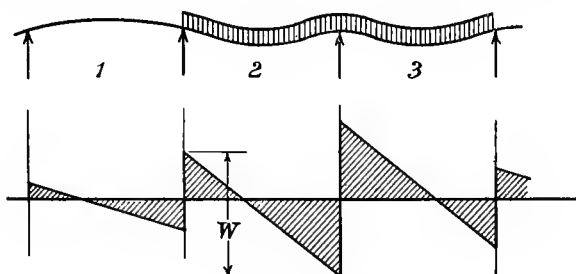
FIG. 83.—Shearing force diagram.
