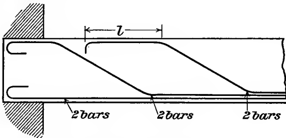
FIG. 39.—Adhesion at supports of beam.
