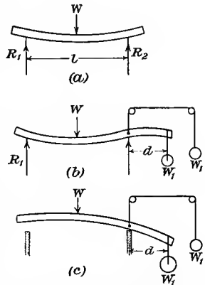
FIG. 62.—Reaction from beam under different conditions.
