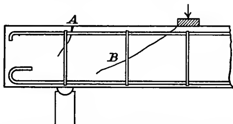
FIG. 42.—Crack due to eccentricity of resistance of hook.
