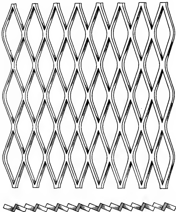
FIG. 115.—Expanded-metal reinforcement.
