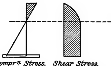
FIG. 46.—Distribution of shear stress across a vertical section of a R. C. beam.
