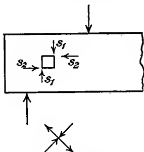
FIG. 45.—Analysis of shear stresses.
