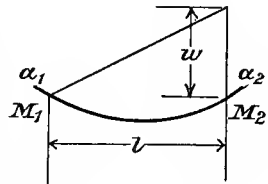
FIG. 156.—Beam under load varying from zero to maximum at one end.
