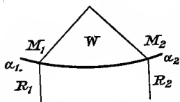
FIG. 140.—One span, triangular loading.
