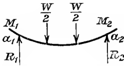
FIG. 142.—One span, two concentrated loads at the third points.
