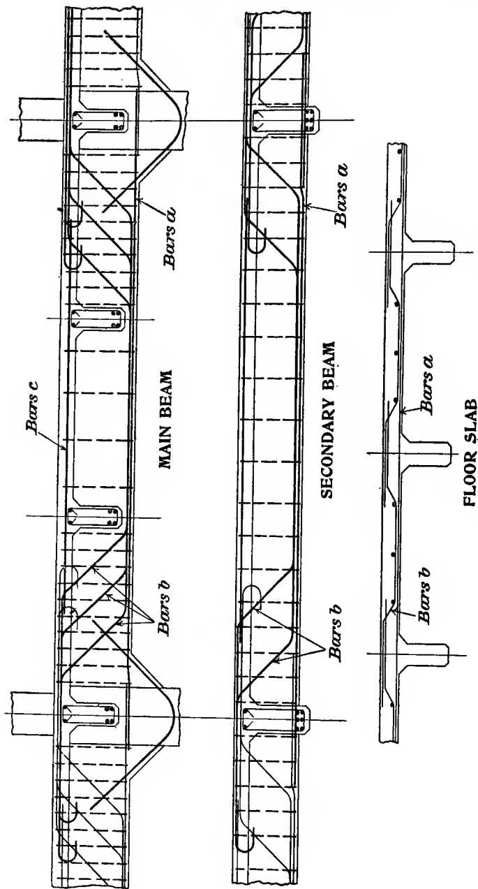
FIG. 2.—Typical arrangement of reinforcement in a continuous beam.
