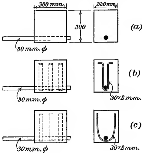
FIG. 37.—Adhesion tests.
