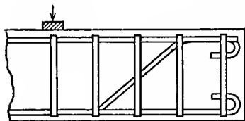
FIG. 53.—Combination of stirrups and bent bars in relation to shear.
