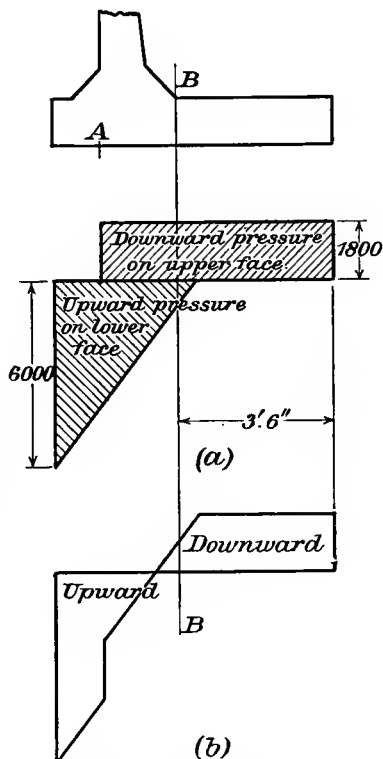
FIG. 130.—Unbalanced pressure on footing.
