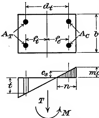
FIG. 26.—Bending and tension with members reinforced on both sides.
